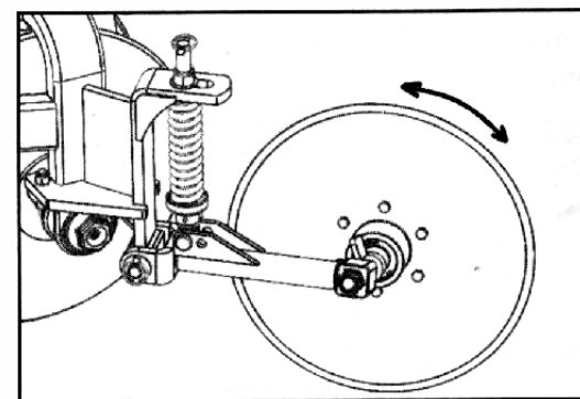
Coulter Disc Assy.
